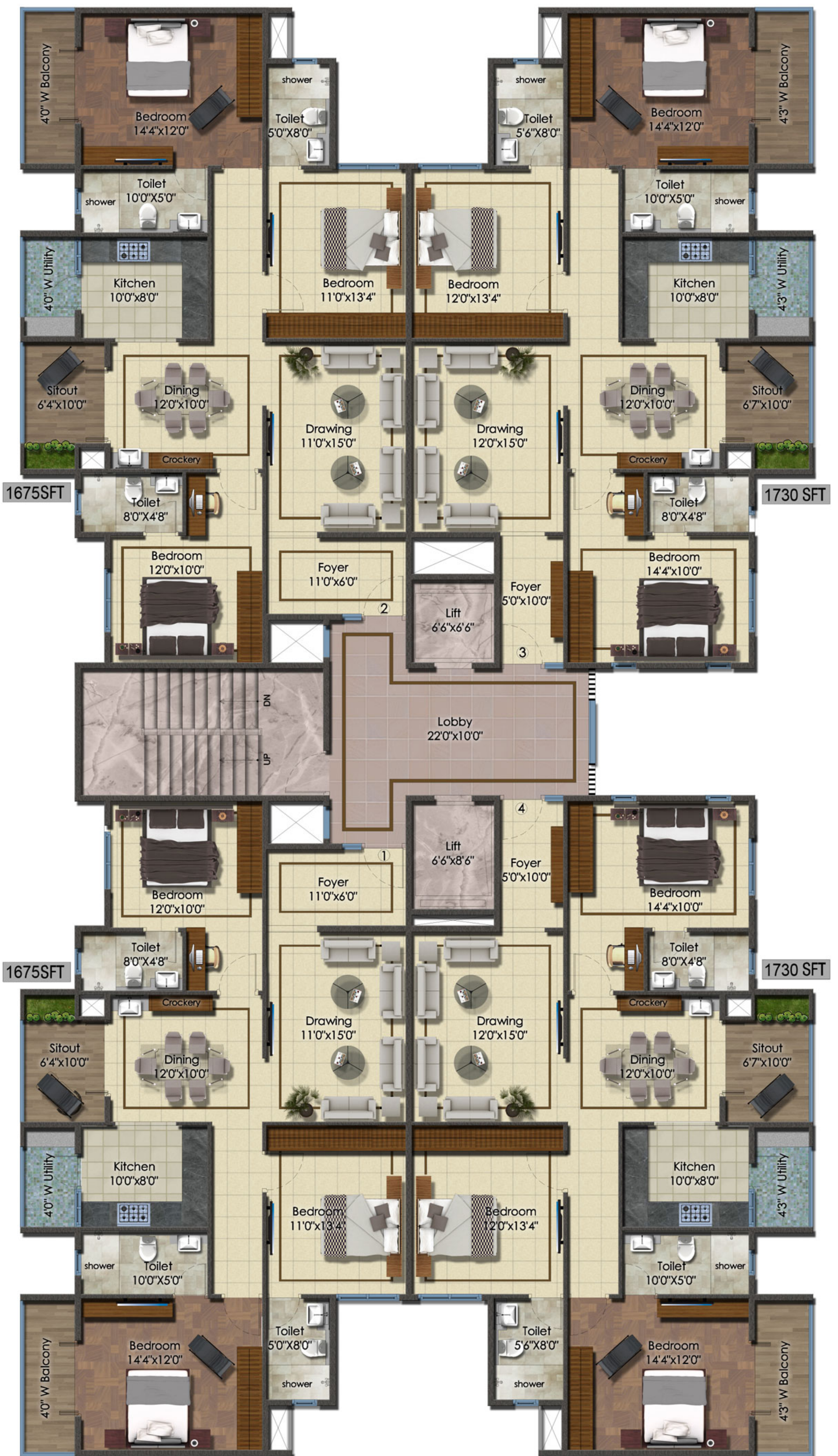
Wing - 3 [2nd to 8th Floor plan]
